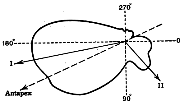
III. Region V. ; centre, R.A. 12 h , Dec. +50°.
